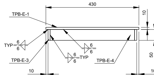
SECTION C-C Scale 1:10
