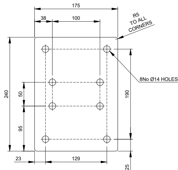
TPC-1 - 10mm THICK Scale 1:5
