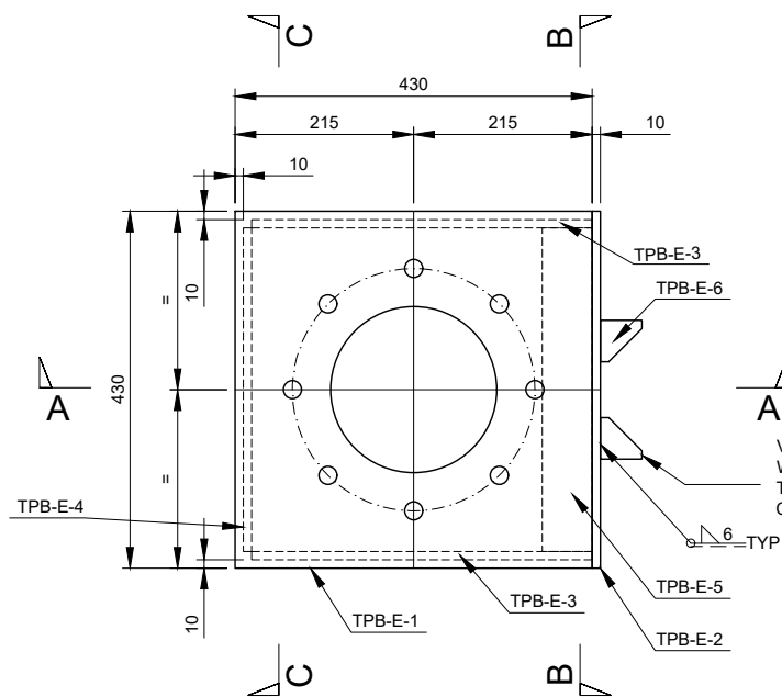
PART TPB-E Scale 1:10
