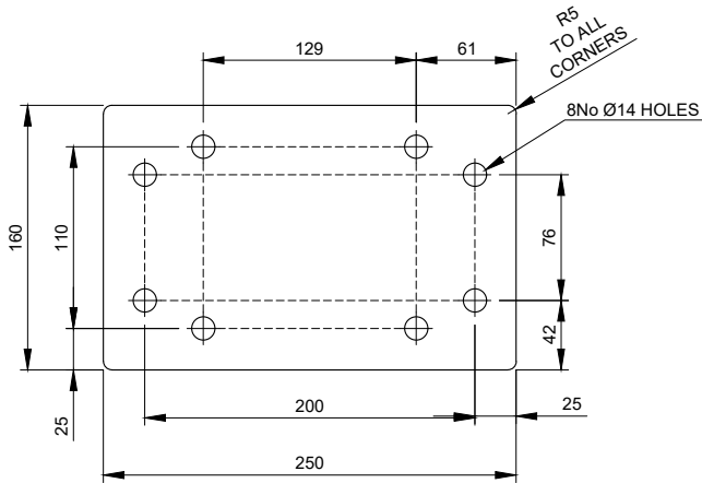
TPC-3 - 10mm THICK Scale 1:5
