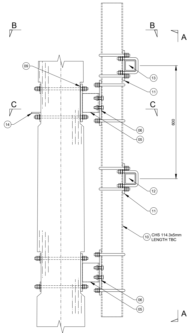
DETAIL H - Rx ANTENNA MOUNT Scale 1:10
