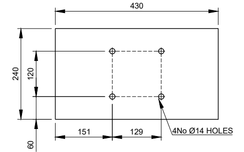
TPB-E-2 - 10mm THICK Scale 1:10
