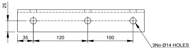
VIEW A-A Scale 1:5
