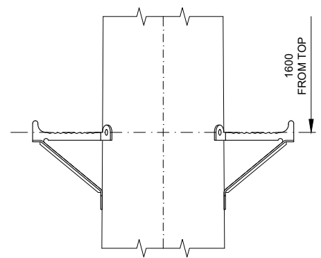
DETAIL D - ANTENNA ACCESS CLIMBING STEP Scale 1:10
