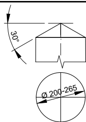
DETAIL A - TIMBER POLE TOP Scale 1:20
