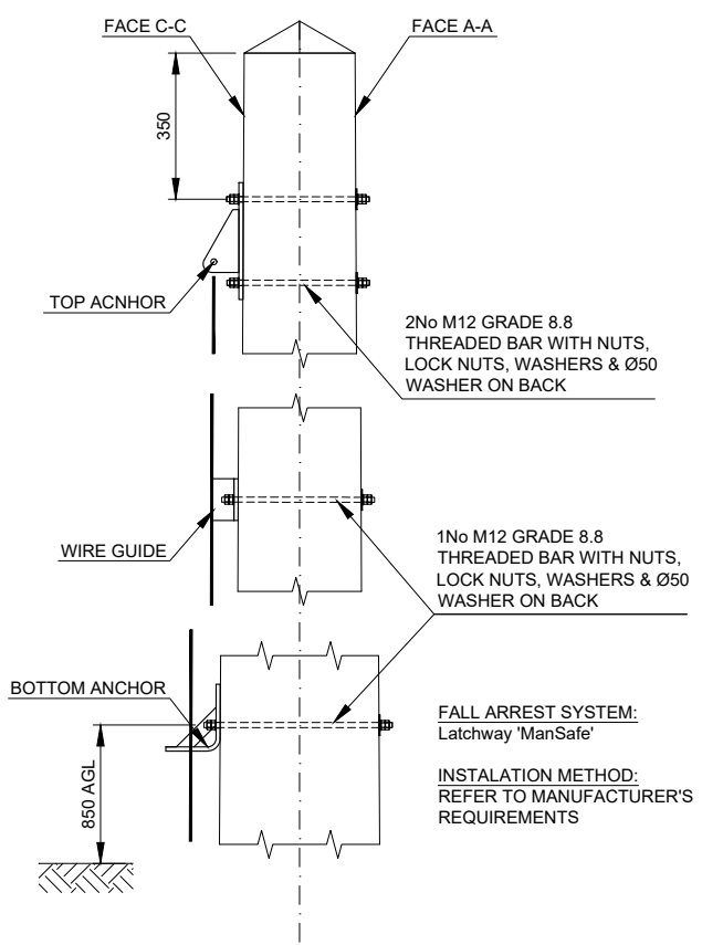
DETAIL B - FALL ARREST SYSTEM Scale 1:20
