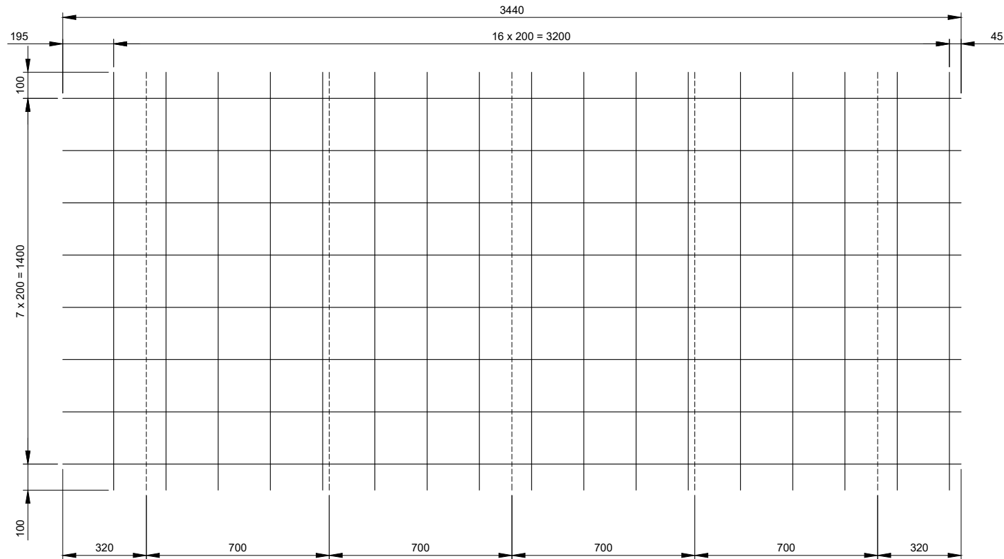
01- A252 MESH 1600x3440mm Scale 1:20
