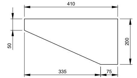
TPB-E-3 - 10mm THICK Scale 1:10
