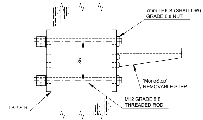
DETAIL F - REMOVABLE CLIMBING STEPS Scale 1:5
