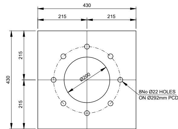
TPB-E-1 - 10mm THICK Scale 1:10
