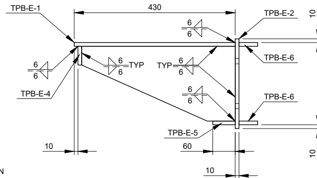
SECTION A-A Scale 1:10
