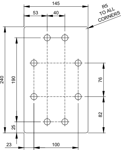
TPC-2 - 10mm THICK Scale 1:5
