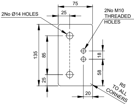
PART TPS-R Scale 1:5
