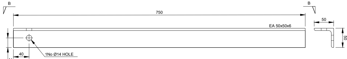
TPA-BR-3 - EA50x50x6 Scale 1:5
