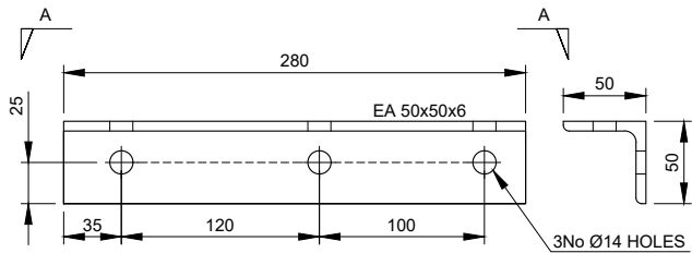
TPA-BR-2 - EA50x50x6 Scale 1:5
