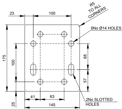
TPA-BR-1 - 10mm THICK Scale 1:5
