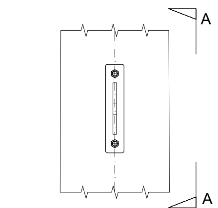
DETAIL C - FALL ARREST ATTACHMENT POINT Scale 1:10
