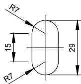
SLOTTED HOLE DETAIL Scale 1:2
