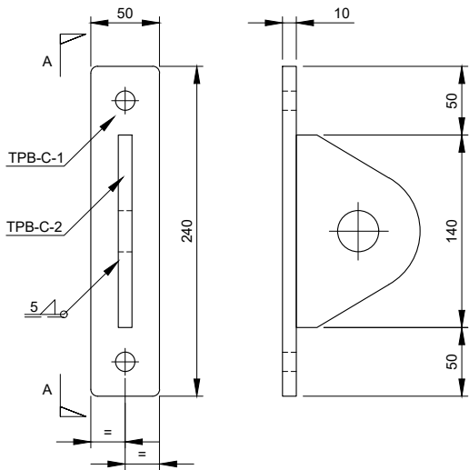
PART TPB-C Scale 1:5
