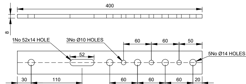
TPA-PD-1 - 8mm THICK Scale 1:5
